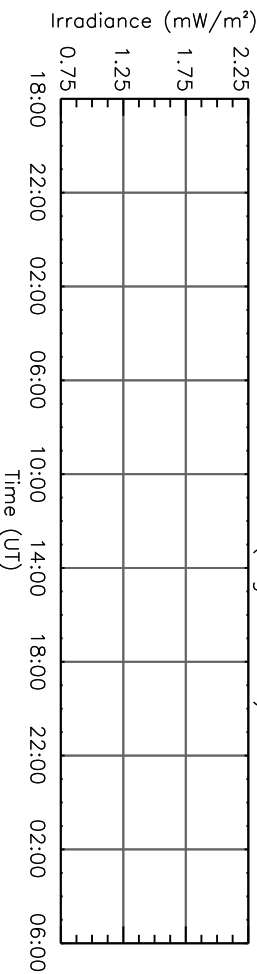
He II 30.38 nm (log T=4.70)
