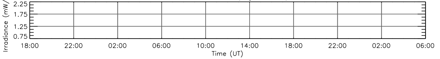
Si XII 49.94 nm (log T=6.29)
