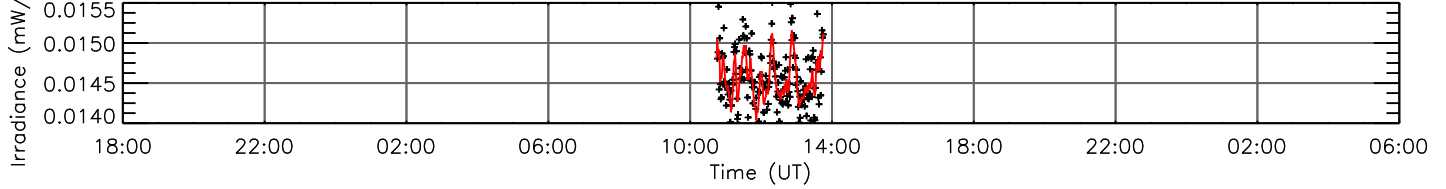
H I 94.97 nm (log T=3.84)
