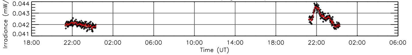
O IV 79.02 nm (log T=5.19)
