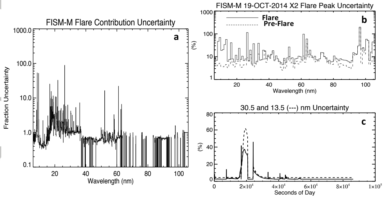
Figure 5. FISIM-M flare uncertainty. a) The fractional uncertainty for the flare model. Note that this is not the sub-daily model uncertainty because the flare contribution is a fraction of the total irradiance and the uncertainties must be weighted accordingly. Panels b and c correspond with an X2 flare observed by EUVM. b) Spectrum uncertainty for flare and pre-flare. The uncertainty increases as the proportion of the total irradiance from the flare increases. c) Example time-dependent uncertainties for the 30.5 nm and 13.5 nm bins.
