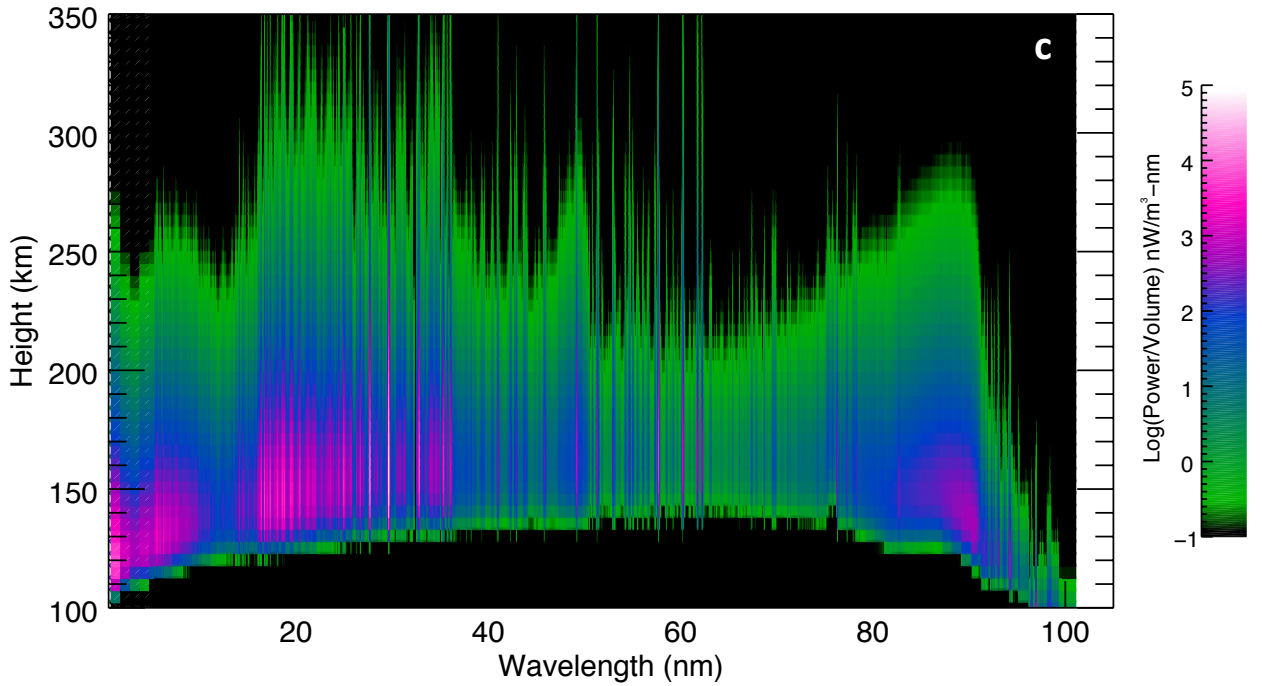
Figure 6. Example results for the FISM-M daily model. Panel a shows the percent decrease from maximum at perihelion to minimum at aphelion during the MAVEN mission in black and solar cycle 23 in red for comparison. Panel b shows the percent decrease from maximum to minimum during a single solar rotation observed in May 2015. Panel c shows the ionization enhancement in the Mars atmosphere due to solar rotation.
