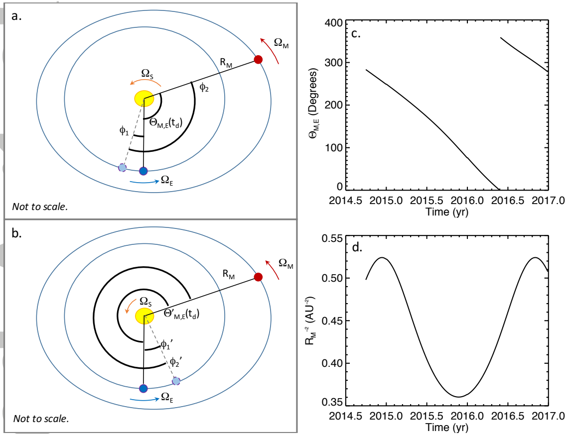
Figure 1. a and b) Geometric definitions used to interpolate Earth measured irradiance proxies to the Mars angular position. t_d is the day when irradiance is needed at Mars. It is found by linearly interpolating irradiance at Earth measured on days t_d - \Delta t_1 and t_d + \Delta t_2 . c) The Mars-Sun-Earth angle and d) the Mars-Sun distance squared as a function of time during the MAVEN mission. See Section 2 for details.
