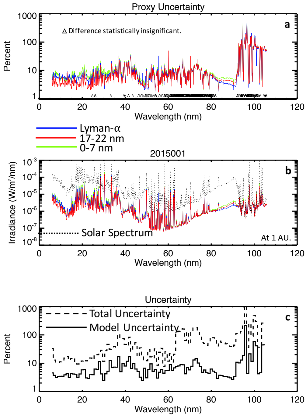
Figure 3. Uncertainties found by comparing FISM-M with SDO EVE measurements. a) Percent uncertainty for each 0.1 nm bin predicted by the three EUVM proxies. The triangles correspond with bins where the F-test found the differences between the smallest and second-smallest uncertainties are statistically insignificant. b) Absolute uncertainty is shown in color and the FISM-M minimum irradiance spectrum is over-plotted with a black dashed line. The values are scaled to 1AU. c) 1 nm signal weighted uncertainty using the minimum model uncertainty for each bin shown in panels a and b. The model and total uncertainties are shown the with black and dashed lines, respectively.
