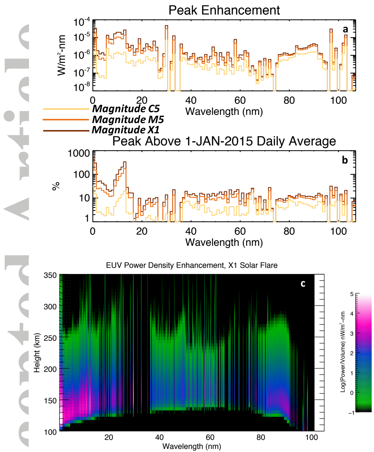
Figure 8. Example FISIM-M flare results for magnitude C5, M5 and X1 flares from 0.1-106 nm. Panel a shows the peak flare irradiance at Mars on 1 January 2015, and Panel b shows the enhancement over the daily average. Panel c shows where in the Mars atmosphere the irradiance enhancement from an X1 flare is deposited.
