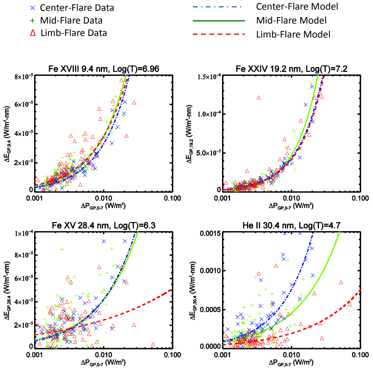
Figure 4. Example bins for the FISM-M gradual-phase fits from MEGS-A. The species, wavelength and Log formation temperature are given at the top of each panel. Power-law fits are found between the MEGS (vertical axis) and the ESP 0-7 nm (horizontal axis) measured peak gradual phase irradiance. The symbols and colors corresponds with flare location on the disk as discussed in the text, and best fit for each population is shown.
