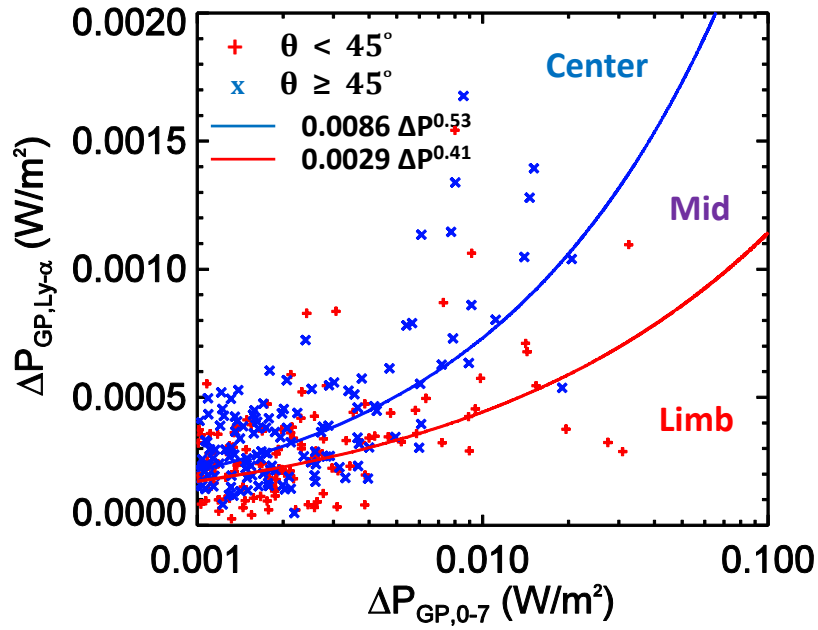
Figure 9. Data and curves used to determine flare location based on the relative response of the EUVM Lyman- \alpha and 0.1-7 nm channels. Fits are found of the training set flares with a 0.1-7 nm signal above 1 \text{ mW/m}^2 for those within 45^\circ from center and those outside of 45^\circ from center. These curves are taken to the boundaries between Center, Mid and Limb flares. Source data to determine this relation are from the ESP 0.1-7 nm and GOES-15 EUVS-E Lyman- \alpha channels.
