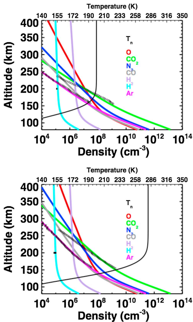
Figure 2. Modeled neutral atmosphere derived using neutral temperature from NGIMS scale heights and constrained to NGIMS densities of CO 2 and Ar. The densities as a function of altitude are generated for the following species: O (red), CO 2 (green), N 2 (blue), CO (grey), H 2 (purple), H (light blue) after coupling to the RT model, and Ar (pink). The neutral temperature profile, T_n , is shown in black with a scale on the top x axis. The black circles show 2 km averaged NGIMS-observed CO 2 and Ar measurements for comparison. A black bar near the H density profile at 200 km indicates the range of H density values at the exobase generated by the RT model for the two cases shown here for (top) active region atmosphere and (bottom) post flare atmosphere.
