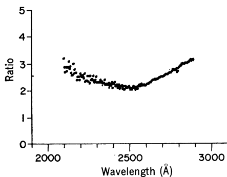
Fig. 5. Ratio of reflectance of polar cap to reflectance of a desert region. This ratio was obtained by dividing the upper spectrum of Fig. 4 by the middle spectrum of Fig. 1.
