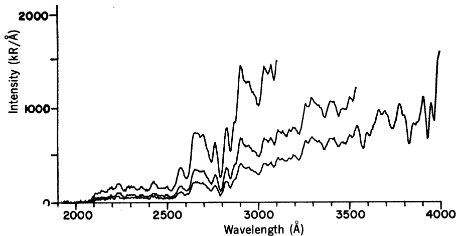
Fig. 1. Mars spectra observed over desert regions. The upper spectrum was obtained while the ultraviolet spectrometer was observing Mars at 4^{\circ}\text{N}, 70^{\circ}\text{W} , with a solar zenith angle \theta_0 of 20^{\circ} , an emission zenith angle \theta of 82^{\circ} , and a phase angle \phi of 63^{\circ} . The middle spectrum was obtained at 1^{\circ}\text{S}, 9^{\circ}\text{W} , with \theta_0 = 47^{\circ} , \theta = 42^{\circ} , and \phi = 62^{\circ} . The lower spectrum was obtained at 18^{\circ}\text{S}, 350^{\circ}\text{W} , with \theta_0 = 65^{\circ} , \theta = 27^{\circ} , and \phi = 90^{\circ} .
