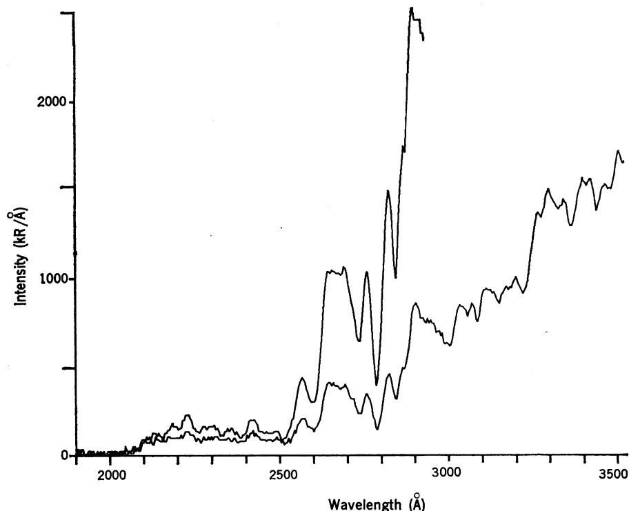
Fig. 4. Comparison of Mars spectrum observed over the polar cap with one observed over desert region. The upper spectrum was obtained while the ultraviolet spectrometer was observing the polar cap at 67°S,5°W, with a solar zenith angle \theta_0 of 41°, an emission zenith angle \theta of 58°, and a phase angle of 55°. The lower spectrum was obtained while the spectrometer was observing the desert at 54°S,29°W, with \theta_0 = 51^\circ , \theta = 50^\circ , and \phi = 55^\circ .
