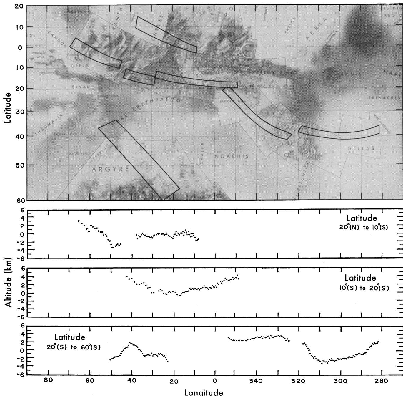
Fig. 3. Elevations of regions on Mars observed from Mariner 6 and Mariner 7. The areas enclosed by heavy lines on the map show the areas observed by the ultraviolet spectrometer. The upper graph gives altitude corresponding to the Mariner 6 observation tracks between 20^{\circ}N and 10^{\circ}S . The middle graph corresponds to the Mariner 6 tracks between 10^{\circ} and 20^{\circ}S , and the lower graph corresponds to the Mariner 7 tracks between 20^{\circ} and 60^{\circ}S .
