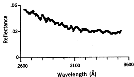
Fig. 2. Ultraviolet reflectance of a desert region. This reflectance was derived from the middle spectrum in Fig. 1.
