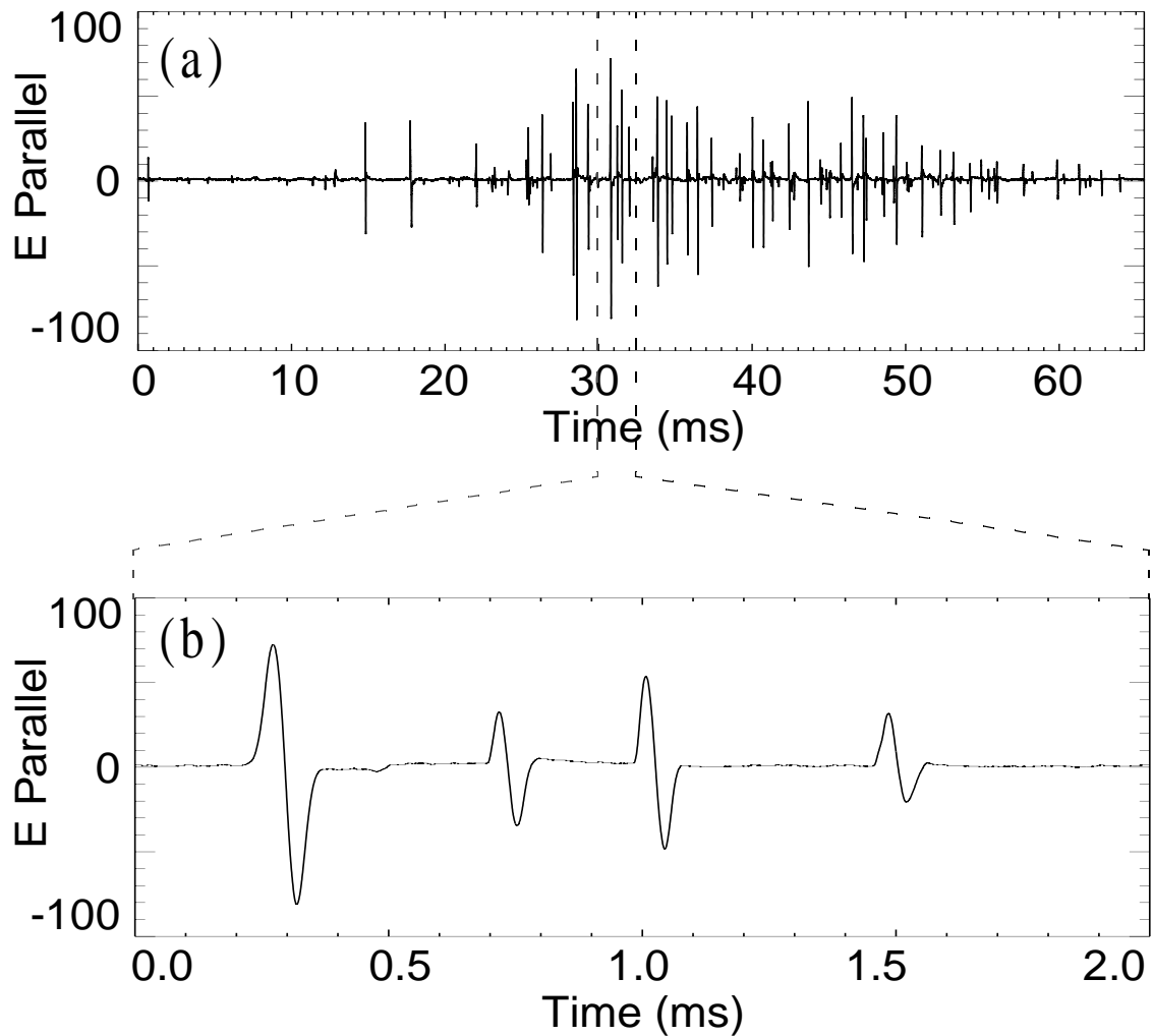
Figure 1. A magnified view of the parallel electric field signal of series of electron holes. The top panel (a) shows \sim 65 ms of data at 0.5 \mu\text{s} resolution. The series of bipolar structures are resolved at this resolution. The bottom panel (b) is a further expanded view of four of the electron holes.
