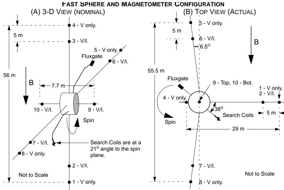
Figure 1. (a) A three-dimensional view of the electric and magnetic field sensors on the FAST satellite as designed. The electric field instrument has eight spherical sensors that are on four wire booms (two each) in the spin plane and two that are on rigid axial booms. All of the spherical sensors can operate in “voltage mode” (marked with “V”) in which they measure the local plasma potential with respect to the payload. The electric field signals are measured by pairs of sensors which form 56 m, 7.7 m, or 5-m dipoles. Six of the ten sensors, marked with “I”, can operate in current mode where the electron current is measured for deriving plasma density. The fluxgate and search coil magnetometers are on ~2-m booms. The search coil assembly is rotated 21° out of the spin plane. (b) The deployed state. The wire boom carrying sensors 3 and 4 did not fully deploy.
