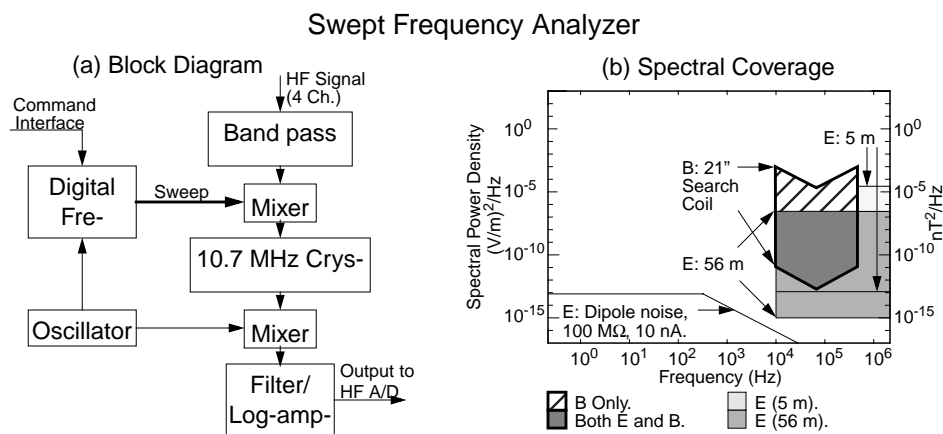
Figure 8. (a) A block diagram of the SFA. Three of the four channels are filtered to 2 MHz and one channel to 4 MHz. The latter channel can be used by the plasma wave tracker by setting the digital frequency synthesizer to a fixed frequency. (b) The spectral coverage and dynamic range of the SFA. The electric field range is from 10^{-15} (V/m) 2 /Hz (56-m dipole) to 10^{-5} (V/m) 2 /Hz (5-m dipole). The 21" search coil has a peak sensitivity at ~65 kHz with a frequency range to ~600 kHz.
