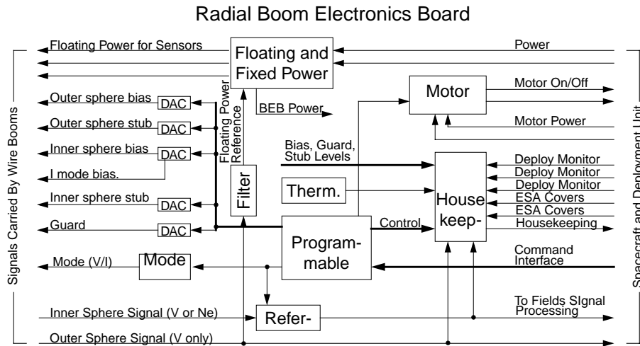
Figure 6. A block diagram of the radial boom electronics board.
