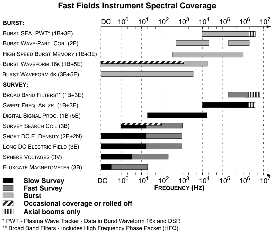
Figure 2. The spectral coverage of Fields Instrument.
