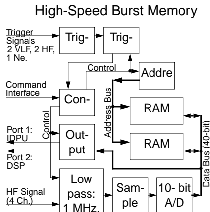
Figure 9. A block diagram of the HSBM. Four high-frequency channels are low-pass filtered then digitized. The data are selected by high- or low-frequency wave event or plasma density cavity by a dedicated trigger system and are stored in a 10 Mbyte RAM. The RAM buffers can be output as waveform data (Port 1) or transferred to the DSP which produces an average of FFTs.
