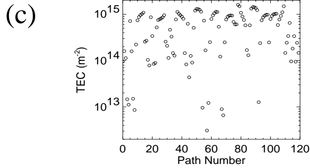
Reconstruction of Plasma Density
