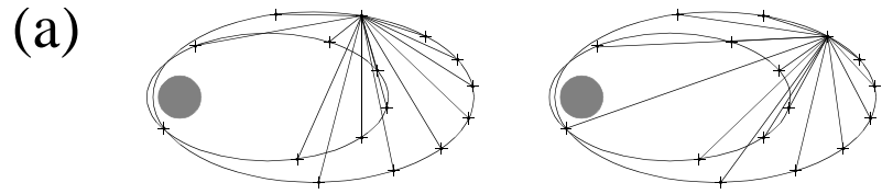
Simulation of Plasma Density
