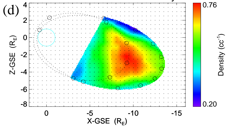
Reconstruction of Plasma Density
