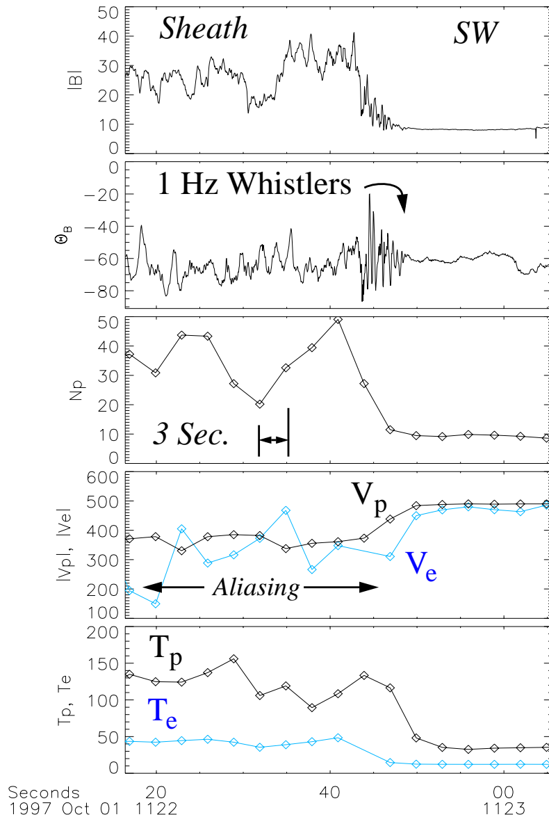
Figure C-3. ‘One Hertz’ whistlers at a bow shock crossing. The upper panels show resolved magnetic field magnitude and latitude, while the bottom panels show 3 second (spin period) Wind/3DP plasma moment data. Solar wind electron and ion velocity moments are well measured, though plasma processes occurring on whistler timescales are highly aliased in spin resolution data.
