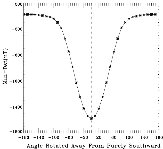
Fig. 3. The minimum values of the modeled Dst if the direction of IMF had been rotated away from purely southward 10^\circ a time, other solar wind parameters kept the same.
