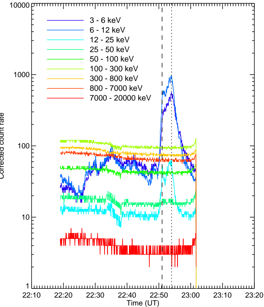
RHessi Quicklook
