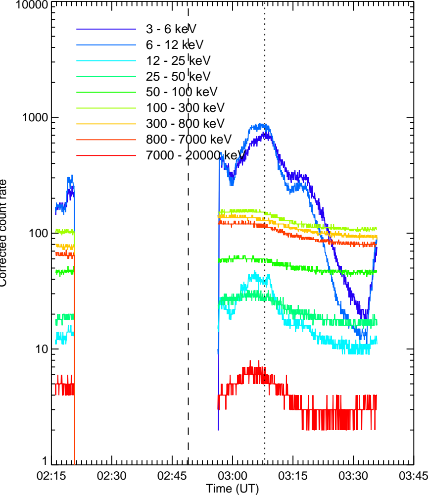
RHESSI Quicklook
