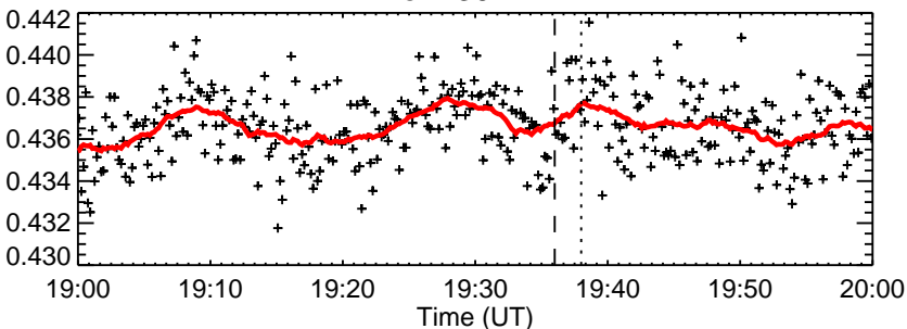
RHESSI Quicklook
