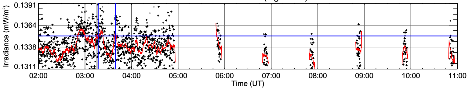
EVE He II 25.6 nm (log T=4.8)
