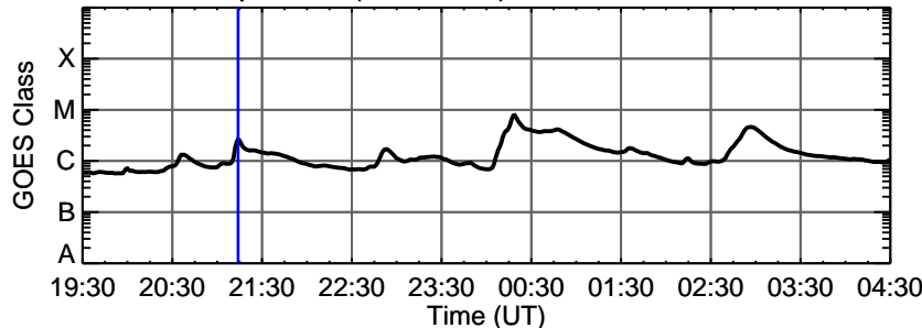
15-Sep-2011 (DOY 258) C2.6 @ 21:14:00 UT
