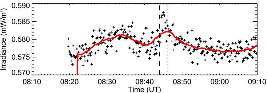
RHESSI Quicklook
