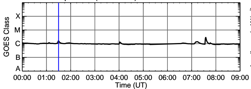
18-Sep-2011 (DOY 261) C1.6 @ 01:30:00 UT
