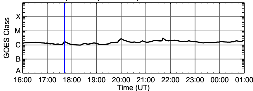
20-Sep-2011 (DOY 263) C1.6 @ 17:42:00 UT
