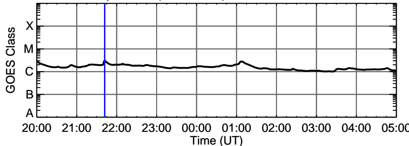
20-Sep-2011 (DOY 263) C3.0 @ 21:42:00 UT
