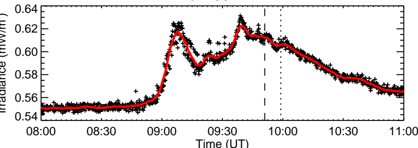
RHESSI Quicklook
