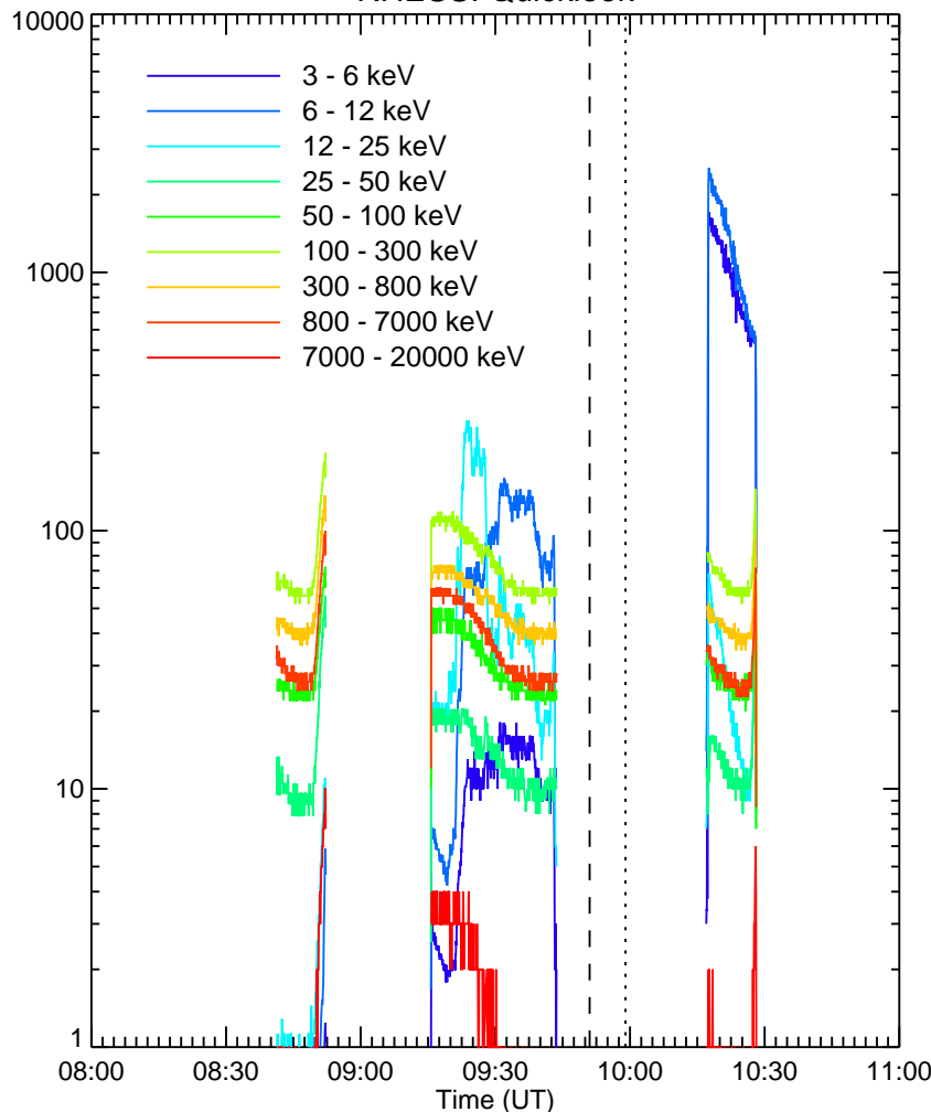
RHESSI Quicklook
