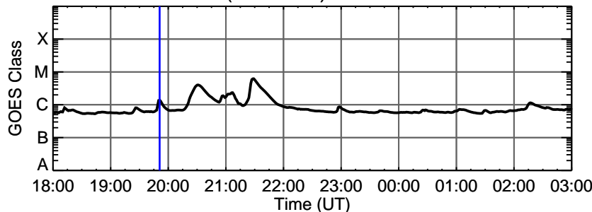
28-Dec-2011 (DOY 362) C1.3 @ 19:51:00 UT
