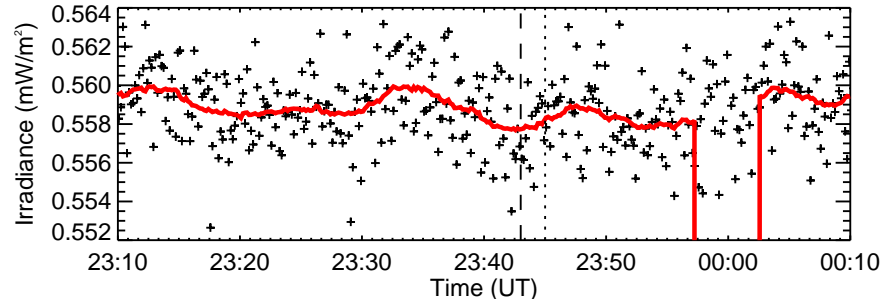
RHESHI Quicklook
