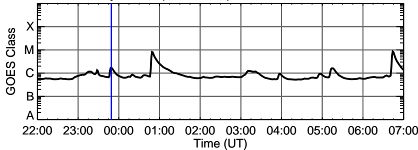
04-May-2013 (DOY 124) C1.7 @ 23:49:00 UT
