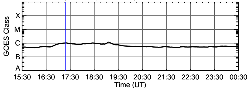
08-May-2013 (DOY 128) C1.0 @ 17:19:00 UT
