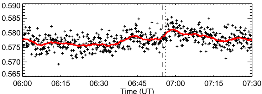
RHESSI Quicklook
