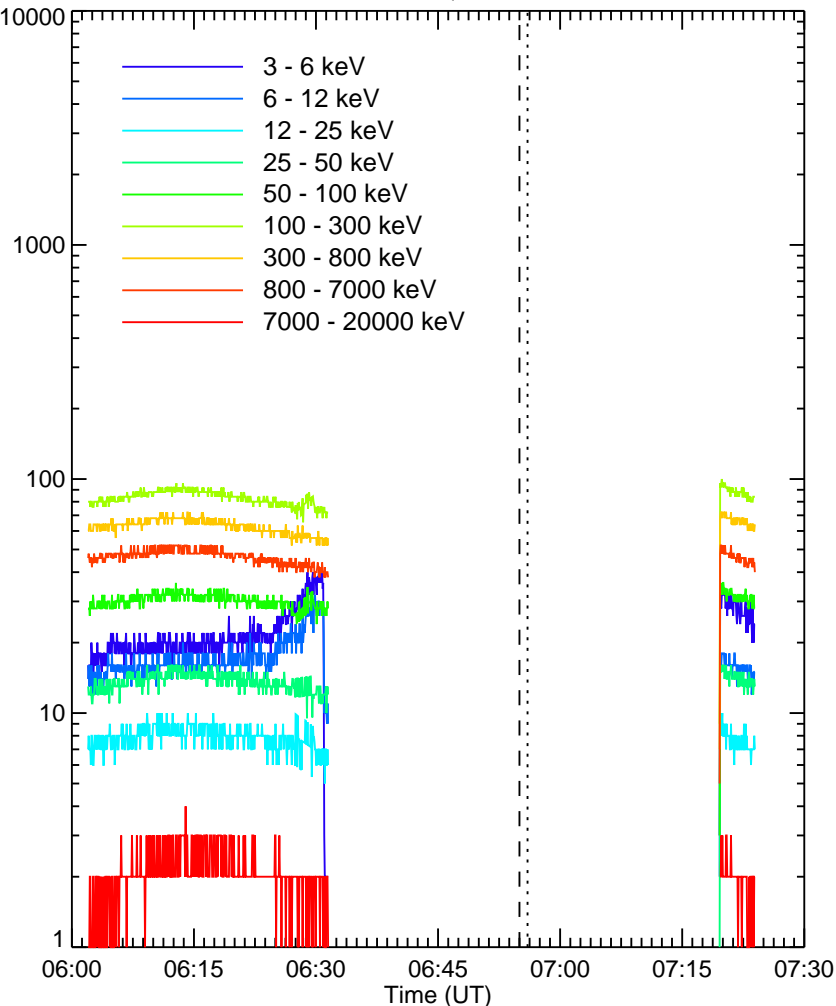
RHESSI Quicklook
