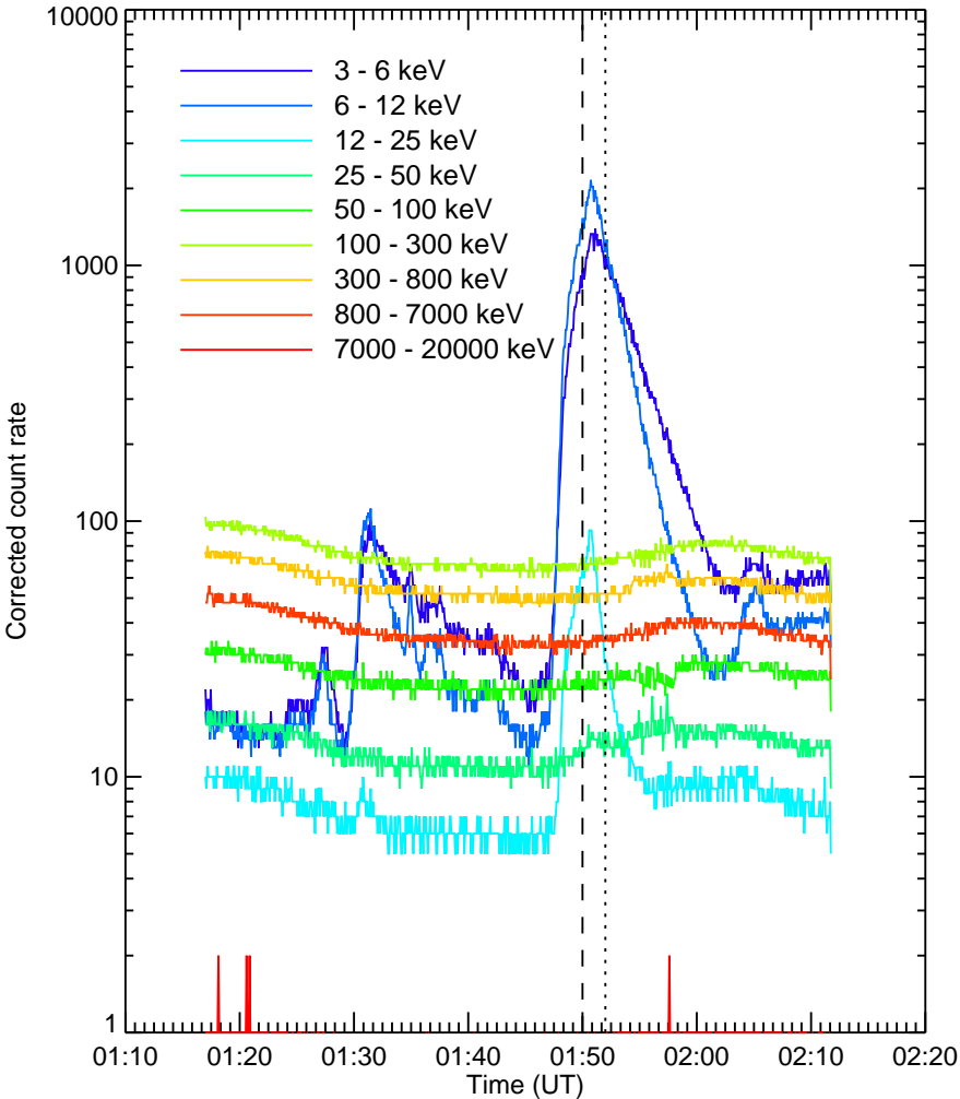
RHESSI Quicklook
