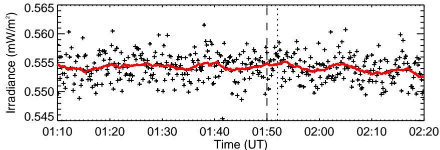
RHESSI Quicklook
