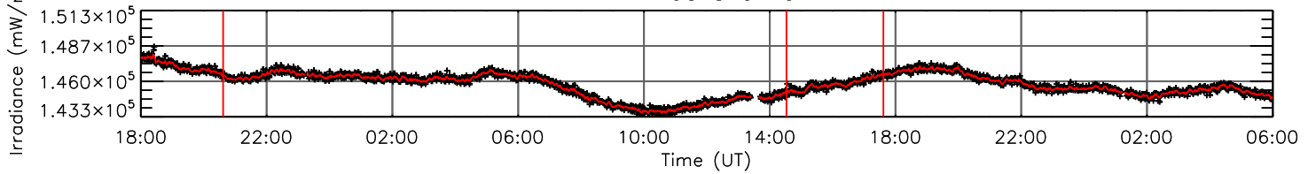
AIA 211 Channel
