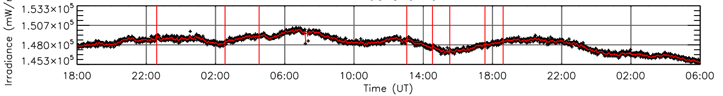
AIA 211 Channel
