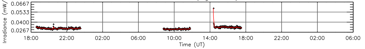
O II 71.85 nm (log T=4.48)
