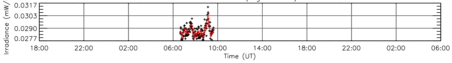
O II 71.85 nm (log T=4.48)
