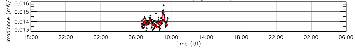
H I 94.97 nm (log T=3.84)
