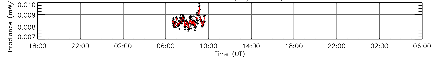
He I 53.70 nm (log T=3.84)
