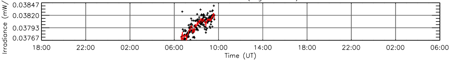
H I 102.57 nm (log T=3.84)
