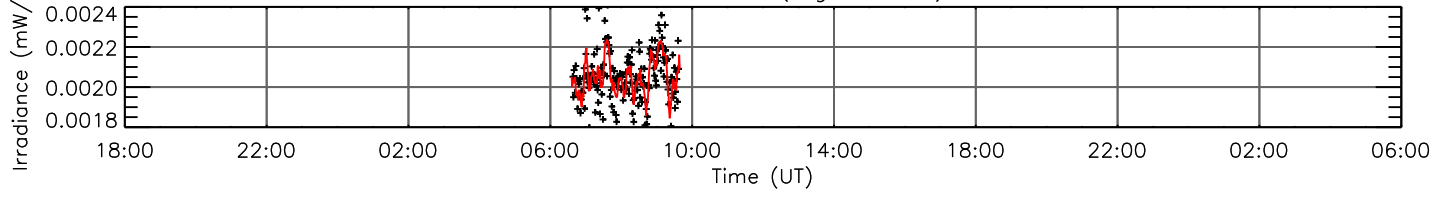
He I 58.43 nm (log T=4.16)
