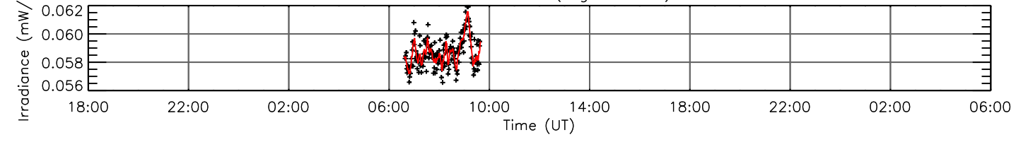
H I 97.25 nm (log T=3.84)
