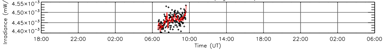
He I 53.70 nm (log T=3.84)
