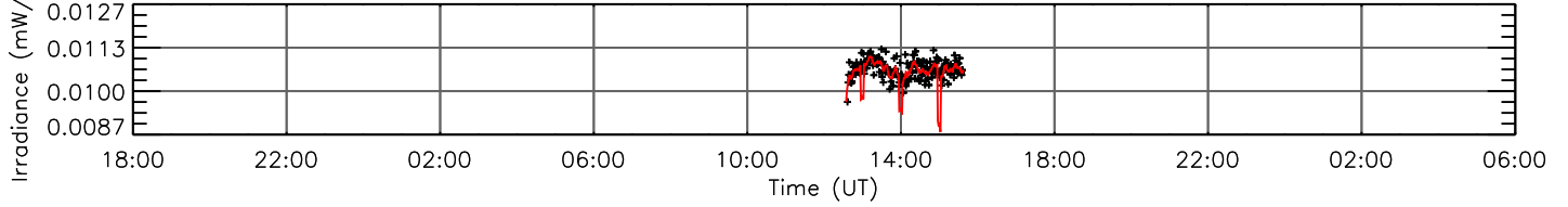
He I 53.70 nm (log T=3.84)
