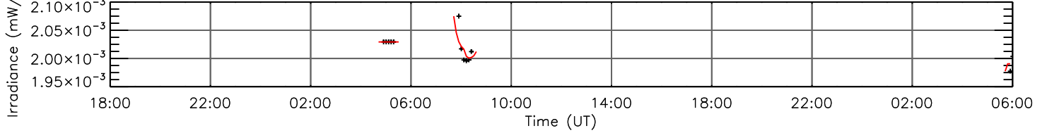
C III 97.70 nm (log T=4.84)
