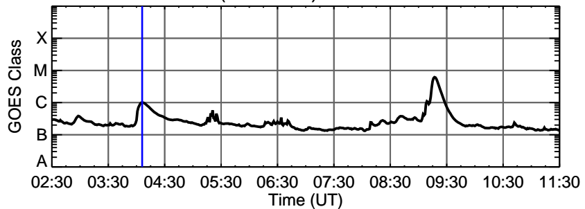
12-Jun-2010 (DOY 163) C1.0 @ 04:06:00 UT
