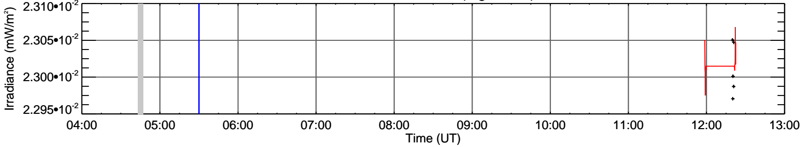
EVE O III 60.0 nm (log T=4.9)
