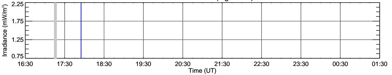
EVE O III 52.6 nm (log T=4.9)
