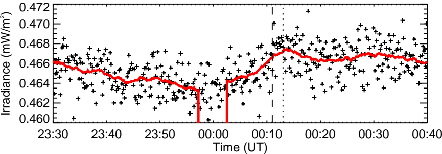
RHESSI Quicklook
