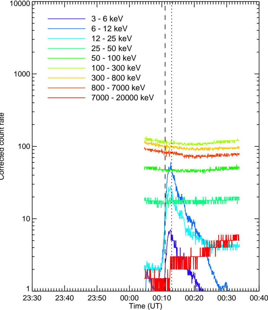
RHESSI Quicklook
