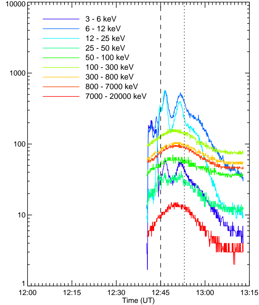
RHESSE Quicklook
