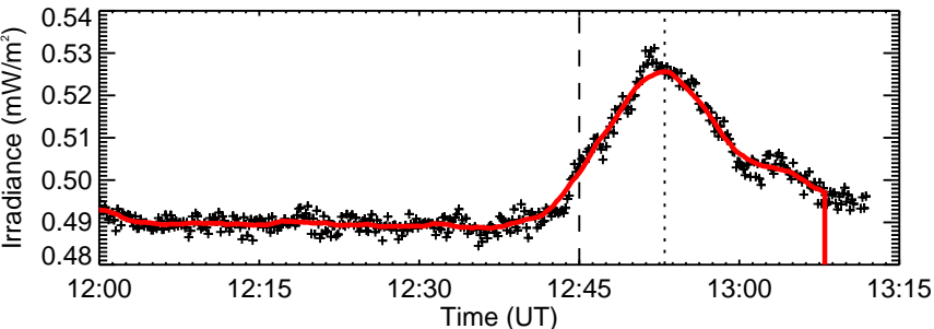
RHESSE Quicklook
