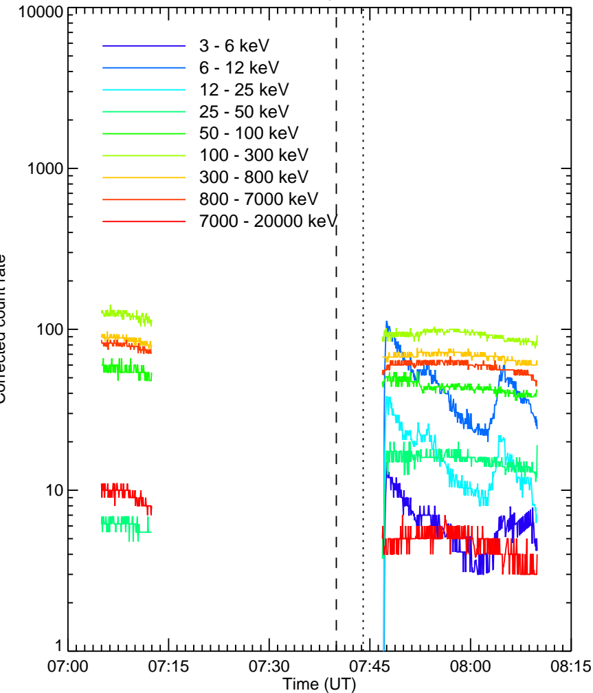
RHESSEI Quicklook
