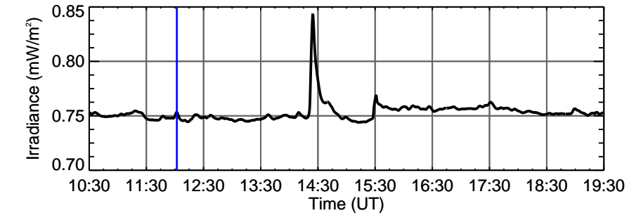
ESP 30.4 nm
