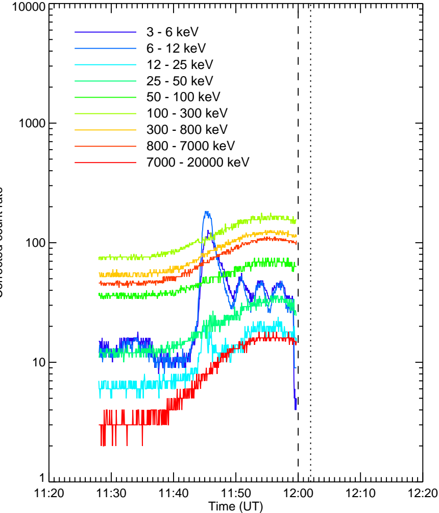
RHESSI Quicklook
