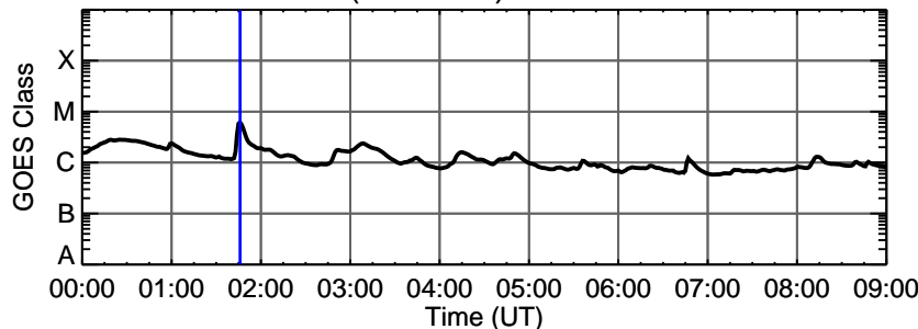
17-Feb-2011 (DOY 048) C6.1 @ 01:46:00 UT
