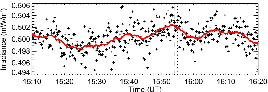
RHESSEI Quicklook
