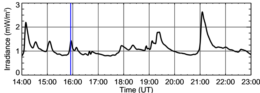
EVE Fe XX 13.3 nm (log T=7.0)
