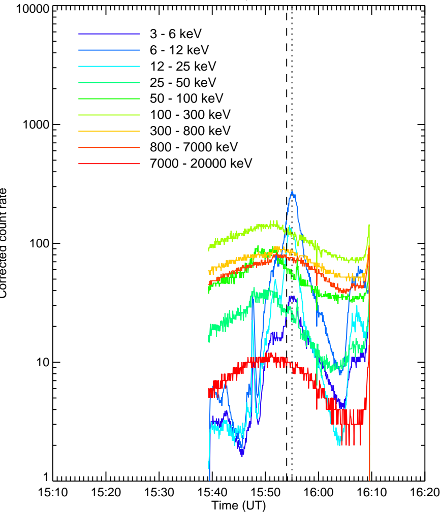
RHESSEI Quicklook
