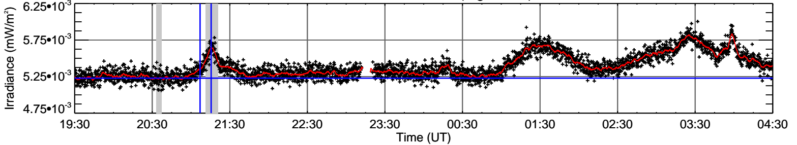
EVE Fe XVI 36.1 nm (log T=6.4)
