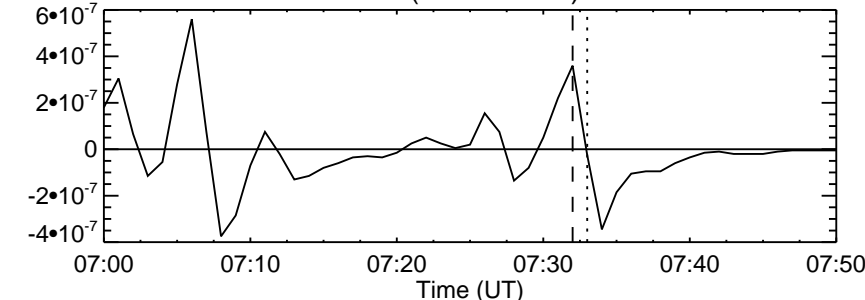
He II 30.4 nm
