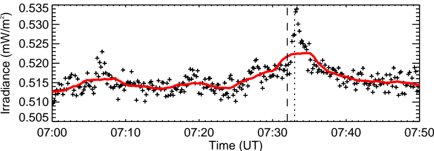
RHESHI Quicklook
