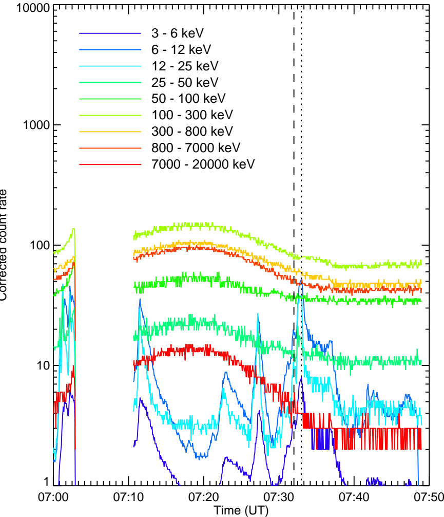
RHESHI Quicklook
