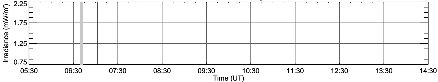
EVE Fe XVI 33.5 nm (log T=6.4)
