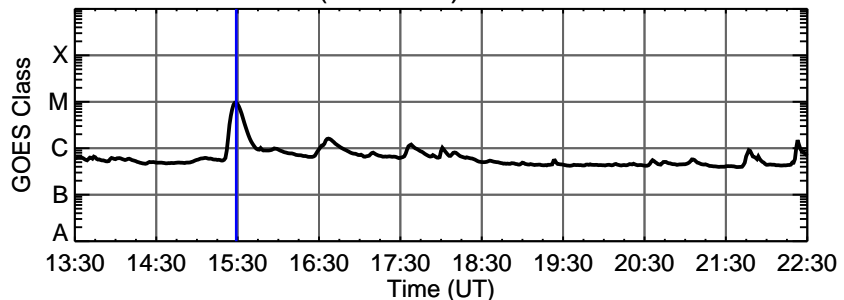
12-Mar-2011 (DOY 071) C9.6 @ 15:29:00 UT
