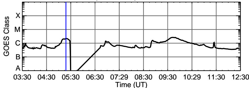
15-Mar-2011 (DOY 074) C2.1 @ 05:18:00 UT
