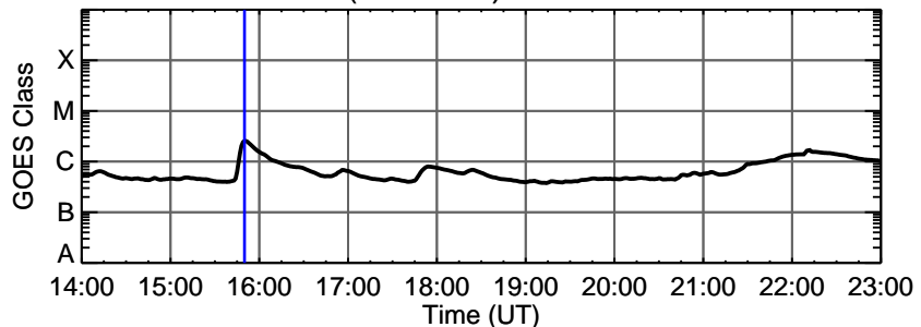
22-Mar-2011 (DOY 081) C2.5 @ 15:50:00 UT
