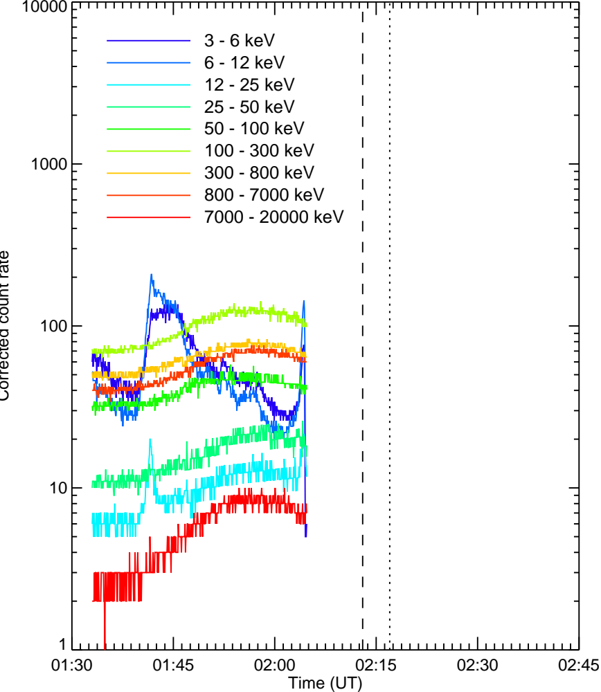
RHESSI Quicklook
